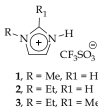
Fig. 6. Protic ILs employed to prepared proton conducting membranes via the polymerization of microemulsions.
