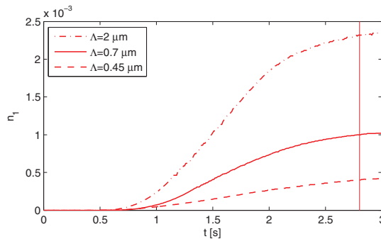
Fig. 12. The grow-curves for different spatial periods of the recording interference field ( I_1 = I_2 = 1.3 \text{ mW}/\text{cm}^2 , t_e = 2.8 \text{ s} ).
