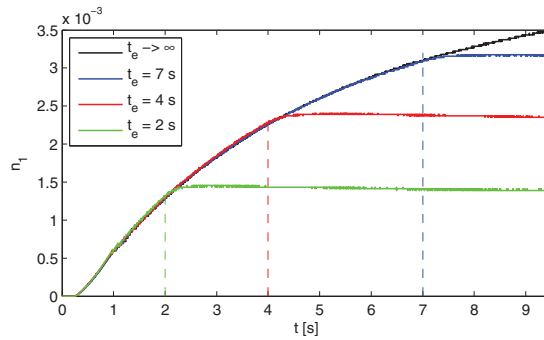
Fig. 13. Post-exposure growth – the exposure was interrupted at t_e = 2, 4, and 7 s ( \Lambda = 0.7 \mu\text{m} and I_1 = I_2 = 3.7 \text{ mW/cm}^2 ).
