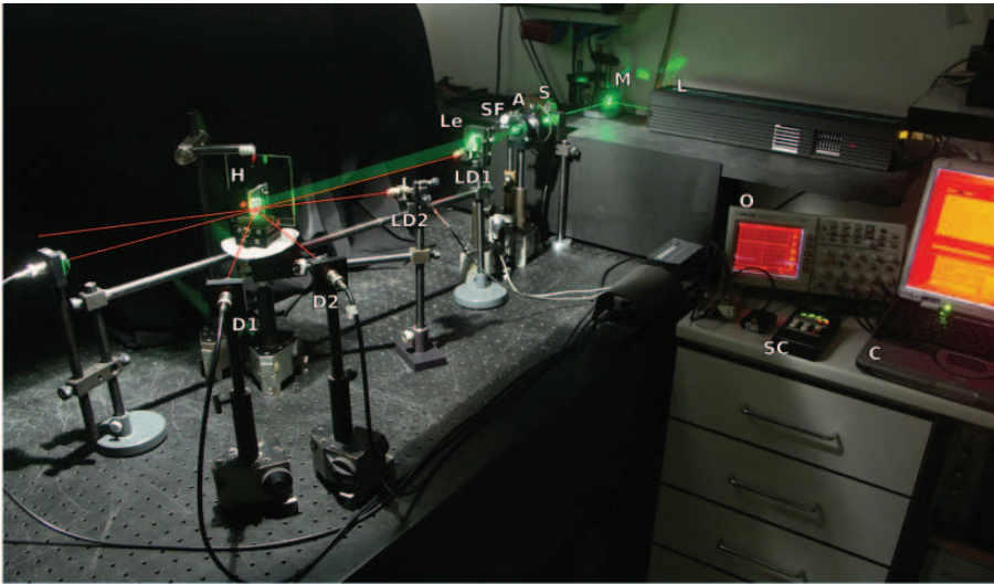
Fig. 7. Experimental setup used for the real-time measurements.
