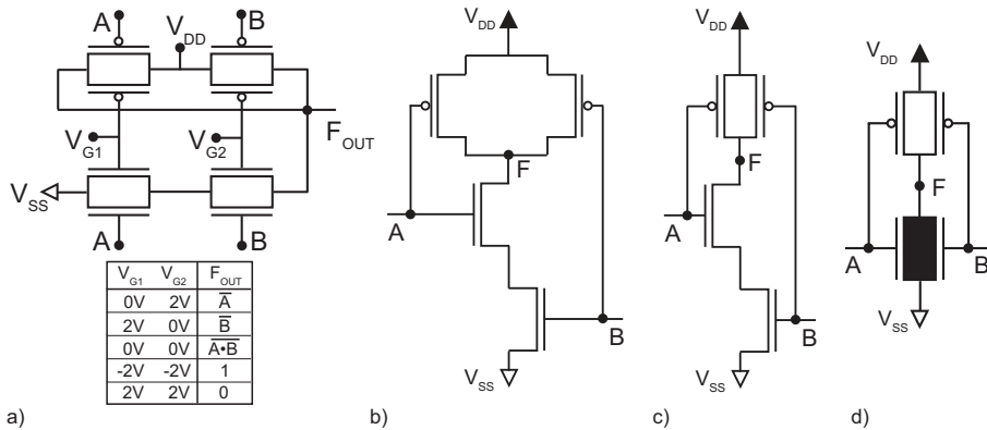
Fig. 15. a) a fine-grain reconfigurable static CMOS digital logic gate realizing five different functions via back gate control by (Beckett, 2008) b) Bulk CMOS NAND implementation, c) hybrid NAND circuit with p-type DG-MOSFET and d) ultra-compact NAND gate realized using a high- V_T n-type DG-MOSFET (filled black) (Chiang et al., 2005)
