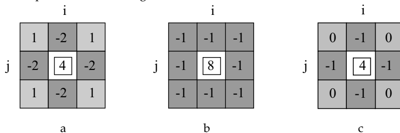
Fig. 1.12 Three different types of Laplacian operators.
