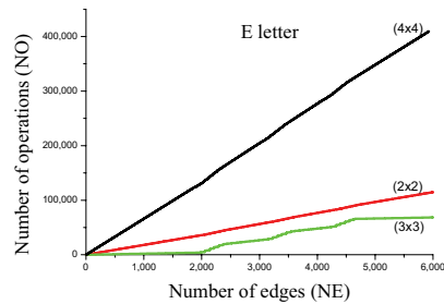
Fig. 1.19 Number of operations versus number of edges for the all algorithms for the shapes of (a) Circle (b) Square (c) E letter.
