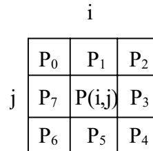
Fig. 1.9b Pixel numbering for 3x3 edge detecting operators.
