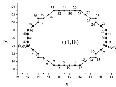
Fig. 2.3 The curve segment of straight line l_1 .
