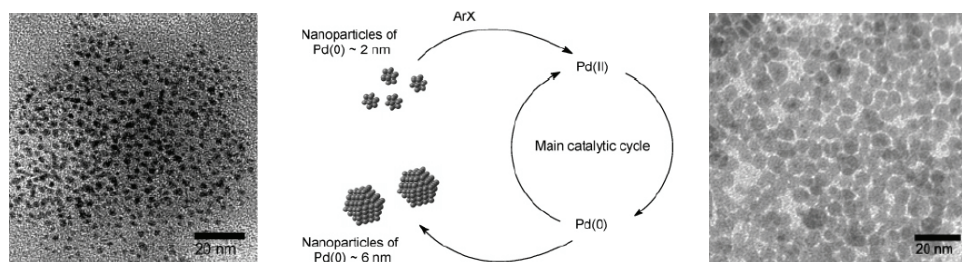
Fig. 1. TEM micrographs of the Pd-NPs in BML.PF 6 : before catalysis ( 1.7 \pm 0.3 nm), left; after catalysis ( 6.1 \pm 0.7 nm), right. The proposed catalytic cycle for the Heck reaction promoted by Pd-NPs is indicated in the middle. Reprinted with permission from reference (Cassol et al., 2005) (Copyright American Chemical Society).
