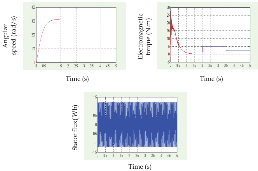
Fig. 11. Robust control under load variation
