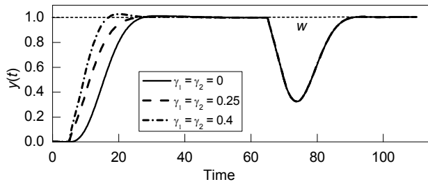
Fig. 3. ITDS: controlled output response ( \tau_d = 5, v = -0.1, \phi = 900 ).
