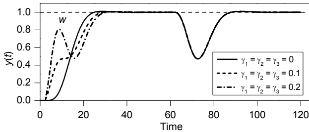
Fig. 15. UFOFITDS: controlled output responses ( \tau_d = 2 , v = -0.05 , \phi = 100 )
