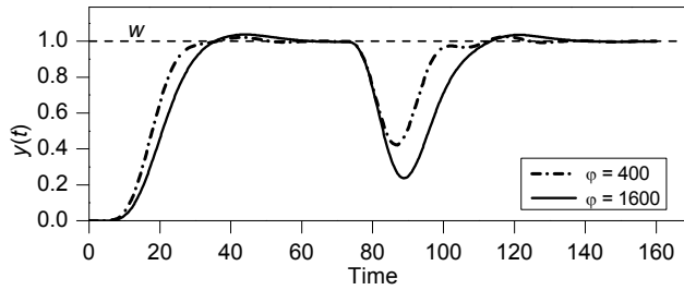
Fig. 14. UFOFITDS: controlled output responses ( \tau_d = 3 , v = -0.025 , \gamma_1 = \gamma_2 = \gamma_3 = 0 )
