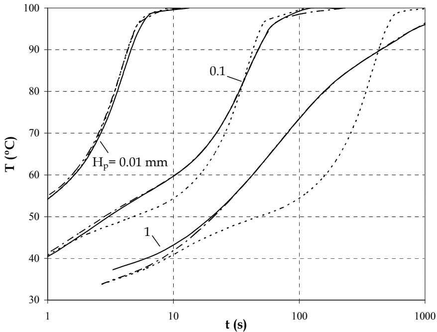
Fig. 15. Predicted temperature at the convective interface considering normal internal resistances (——), null thermal and mass resistances (----- approach A) and null thermal resistance (-·-·-·- approach B)
