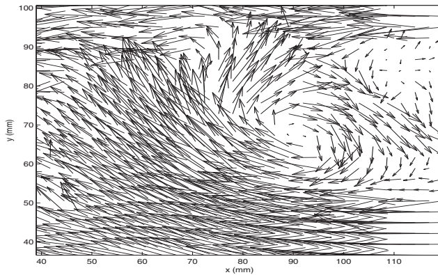
Fig. 3. Computed velocity vectors for a sample snapshot
