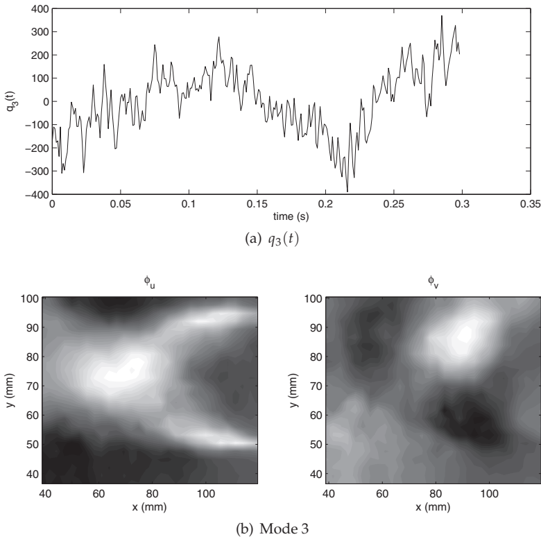
Fig. 9. The third mode for test 1
