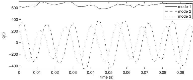
Fig. 11. Variation in time of the three retained generalized coordinates, Test 2
