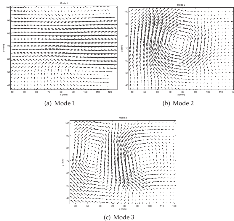
Fig. 16. Vector plots of the first three mode shapes
