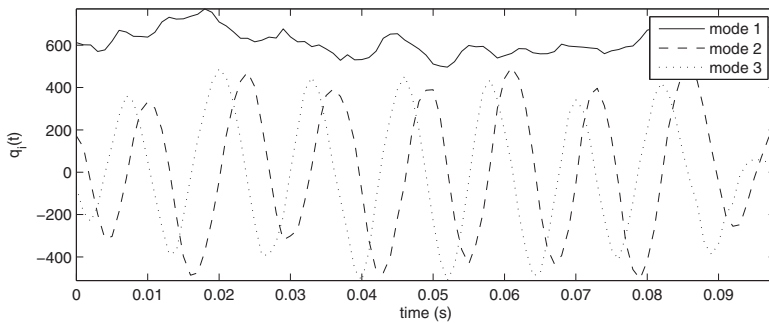
Fig. 12. Variation in time of the three retained generalized coordinates, Test 3
