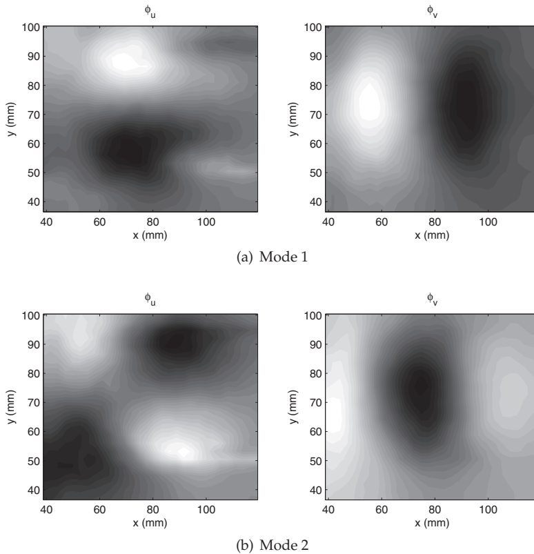
Fig. 7. The first two mode shapes for test 1
