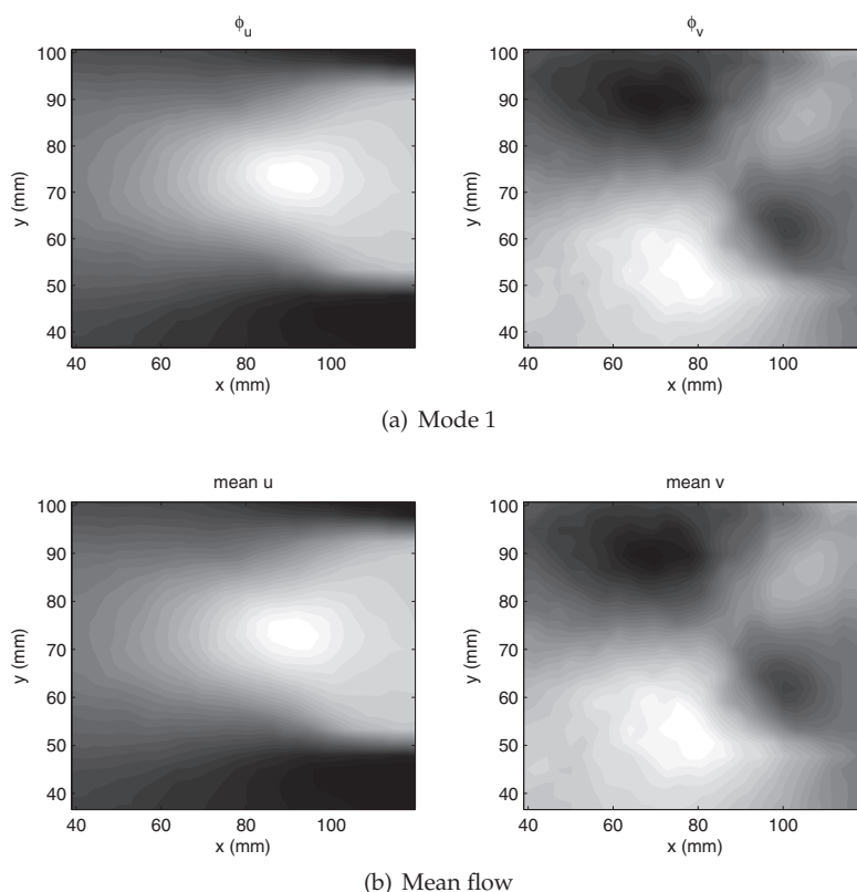
Fig. 10. The first mode shape for test 2 (top) compared to the mean flow (bottom)
