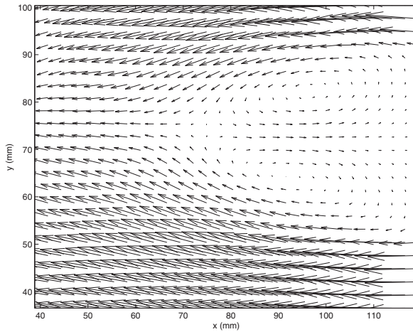
Fig. 5. Mean flow vectors for test 1
