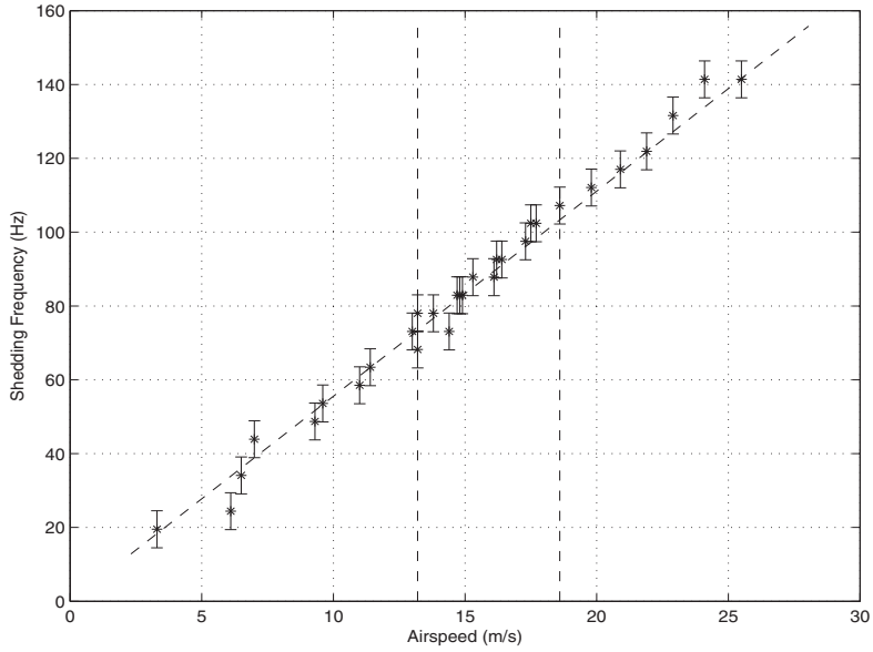
Fig. 4. Comparison of estimated frequencies to theoretical frequencies
