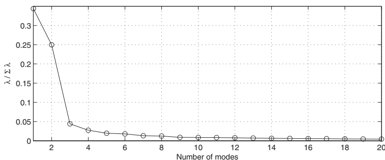
Fig. 6. Eigenvalue ratios for the first 20 eigenvalues for test 1
