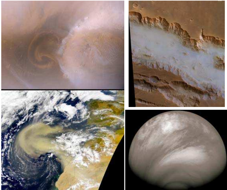
Fig. 1. Left upper and lower; satellite photographs of Mars and Earth, North Africa respectively, showing dust storms and clouds. (Courtesy NASA/JPL-Caltech). Right upper fog in Mars, Valles Marineris taken by the High Resolution Stereo Camera (HRSC) on board ESA's Mars Express spacecraft, Right lower; acid haze seen amongst the thick clouds of Venus, photographed by the ESA's Venus Express spacecraft.
