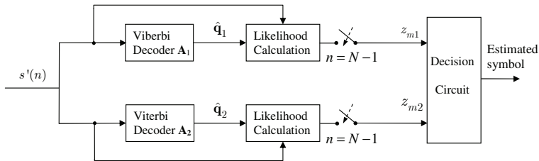
Fig. 13. Receiver for MMLCSK using two maps.
