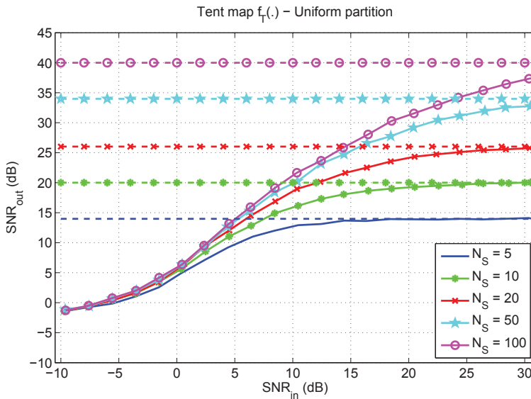
Fig. 10. SNR_{out} of MVA for an orbit of length N = 10 using different numbers of partition intervals N_S . The generating map is f_T(\cdot) . Performance limits of Eq. (46) are indicated by dashed lines.
