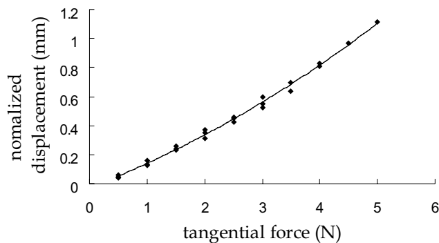
Fig. 8. Relation between normalized displacement and tangential force.
