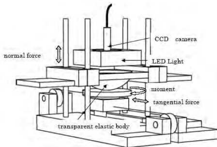
Fig. 3. Experimental setup for the sensor.
