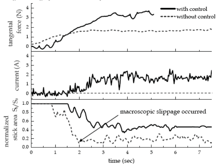
Fig. 15. Result of stick area control: Comparison between with and without control.
