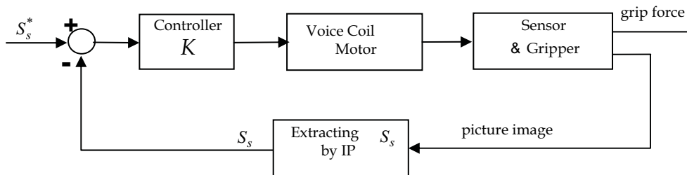
Fig.14. Block diagram of grip force control system.
