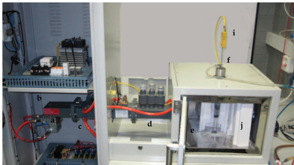
Fig. 1. Photographs of singlemode (upper) and multimode (lower) microwave ovens at INCAR ( www.incar.csic.es ) showing: a) magnetron; b) waveguide; c) circulator with reflected power meter; d) tuning screws; e) resonant cavity; f) reactor; g) terminator with transmitted power meter; h) infrared optical pyrometer; i) thermocouple; and j) insulating material
