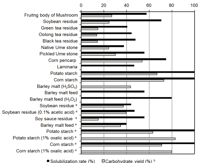
Fig. 14. Weight loss and carbohydrate yield after microwave irradiation (% w/w) of unutilized biomass from food, agricultural and fishery industries. a Results obtained by using continuous flow system. b Data on weight basis.
