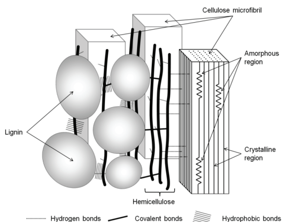
Fig. 11. Schematic illustration of lignin-polysaccharide network
