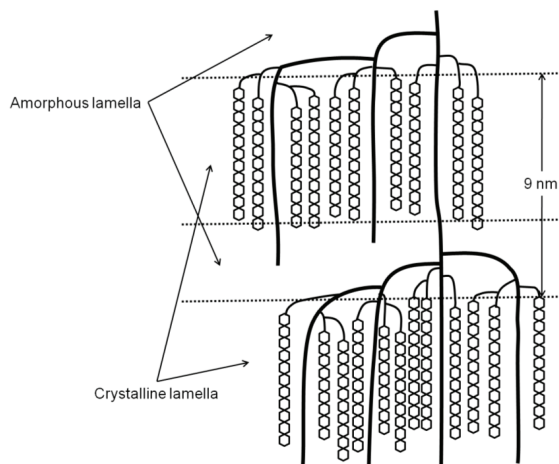
Fig. 3. Schematic illustration of lamellar structure of a starch granule.
