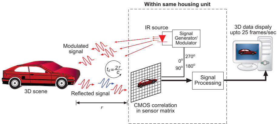
Fig. 2. Basic principle of TOF 3D imaging system.
