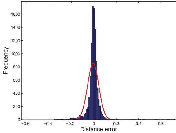
Fig. 5. Statistical distribution of planar feature data points derived from experimental data documented in Section 6.
