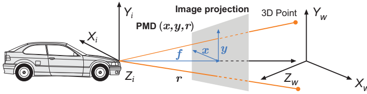
Fig. 3. Time-of-Flight sensor geometry
