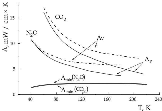
Fig. 3. Isochoric (dashed lines) and isobaric (solid lines) thermal conductivities \Lambda of CO_2 and N_2O .
