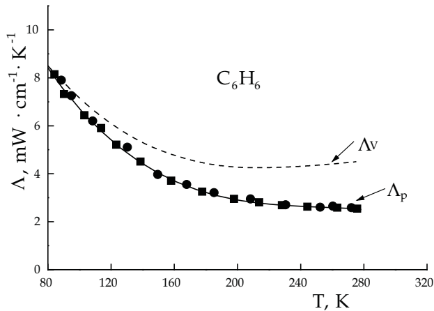
Fig. 10. Isochoric ( V_m=70.5 \text{ cm}^3/\text{mole} ) and isobaric thermal conductivity of solid \text{C}_6\text{H}_6 .
