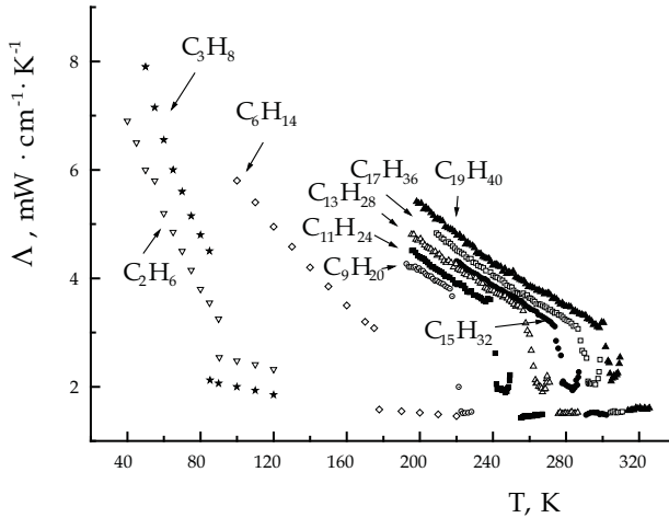
Fig. 11. Isobaric thermal conductivity of some n -alkanes.
