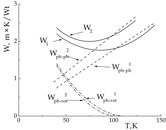
Fig. 7. Contributions of phonon-phonon scattering W_{ph-ph} and phonon scattering by rotational molecule excitations W_{ph-rot} to the total thermal resistance W of solid methane samples having molar volumes 30.5 (1) and 31.1 (2) \text{cm}^3/\text{mole} .
