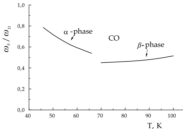
Fig. 16. The \omega_0/\omega_D ratio upon temperature.
