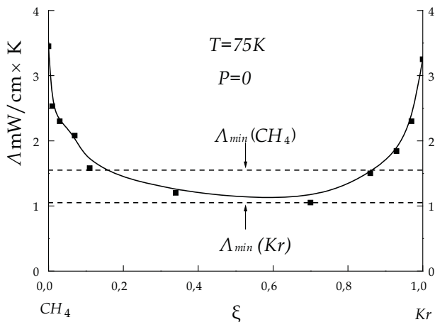
Fig. 13. The concentration dependence of the thermal conductivity of solid solution (CH_4)_{1-\xi}Kr_{\xi} at T=75K and P=0 . The horizontal lines are \Lambda_{min} of pure Kr and CH_4 under the same conditions calculated by Eq. 4.
