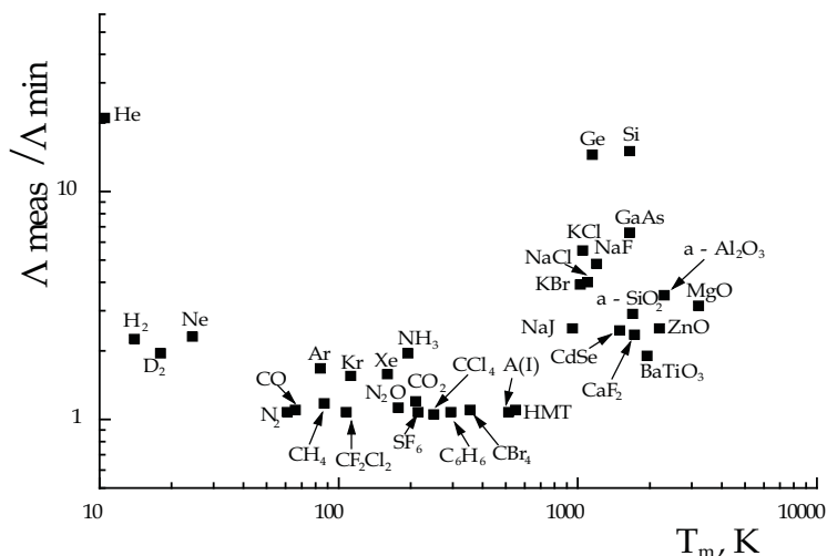
Fig. 1. The ratio \Lambda_{meas}/\Lambda_{min} immediately below the corresponding melting temperatures ( T_m ) versus T_m for crystals with different types of chemical bonds.
