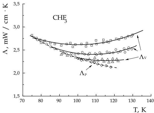
Fig. 8. The isochoric thermal conductivity of three solid \text{CHF}_3 samples of different densities. Solid lines show smoothed values of isochoric thermal conductivity. Dashed line and rhombus are for the thermal conductivity of a free sample.
