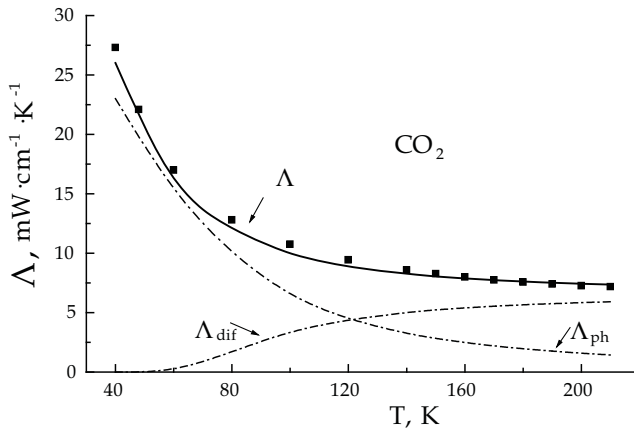
Fig. 15. Contributions \Lambda_{ph} and \Lambda_{dif} for CO_2 sample with molar volume 25.8 \text{ cm}^3/\text{mole} .
