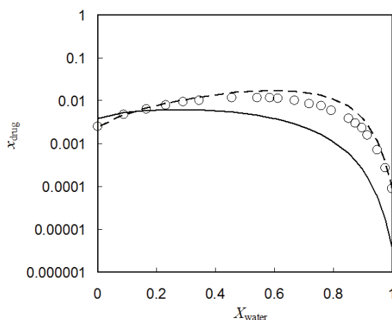
Fig. 15. Solubility of sulphisomidine in the solvent of water and dioxane at 298.15 K from PR+COSMOSAC (solid line) and PR+COSMOSAC+ G^{\text{dspotr}} (dashed line). Experimental data (Martin et al., 1985) are shown in open circles. The x-axis X is the solvent fraction in the solute free solvent mixtures.
