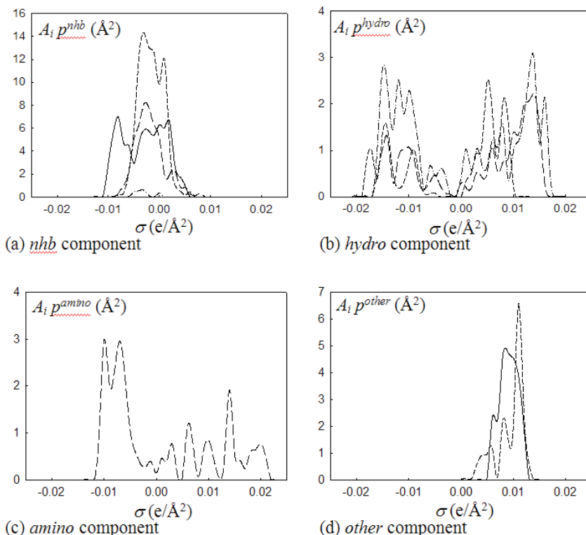
Fig. 3. The sigma profiles for four representative compounds: acrylonitrile (solid line), monoethanolamine (long dashed line), isobutyric acid (short dashed line), and water (dashed-dotted line). A_i is the molecular surface area of species i .
