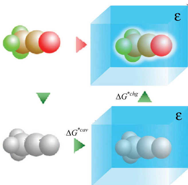
Fig. 1. The solvation process can be separated into two steps: (1) creating a cavity to size of the solute ( \Delta G^{*cav} ) and (2) placing the solute into the cavity ( \Delta G^{*chg} )
