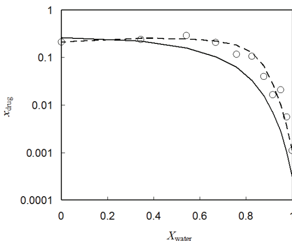
Fig. 14. Solubility of acetanilide in the solvent of water and dioxane at 293.15 K from PR+COSMOSAC (solid line) and PR+COSMOSAC+ G^{\text{dsporr}} (dashed line). Experimental data(Bustamante et al., 1998) are shown in open circles. The x-axis X is the solvent fraction in the solute free solvent mixtures
