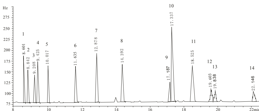
Fig. 2. 1. \alpha -HCH, 2. Hexachlorobenzene, 3. \beta -HCH, 4. \gamma -HCH, 5. \delta -HCH, 6. Heptachlor, 7. Aldrin, 8. Heptachlor expoxide, 9. 4,4'-DDE, 10. Dieldrin, 11. Endrin, 12. 4,4'-DDD, 13. 2,4'-DDT, 14. 4,4'-DDT.
