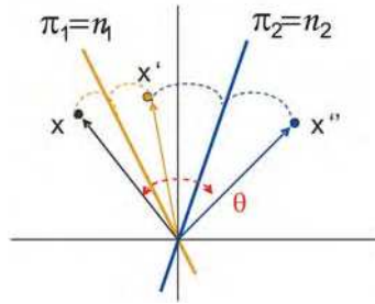
Fig. 9. Reflection about nonparallel planes.
