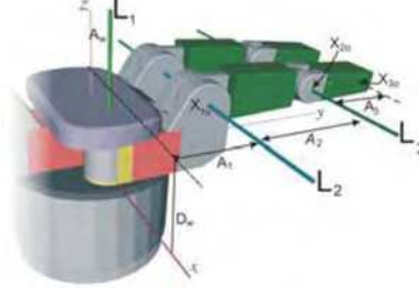
Fig. 15. Barrett hand hypothetical position.
