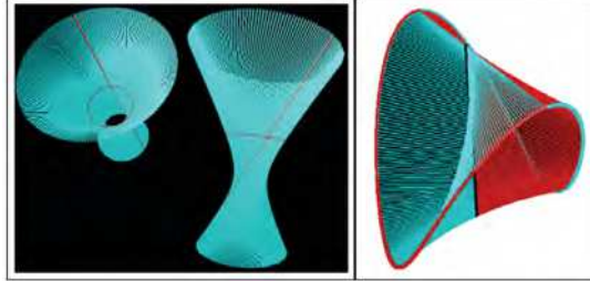
Fig. 13. (a) Hyperboloid as the rotor of a line. (b) The Plücker conoid as a ruled surface.
