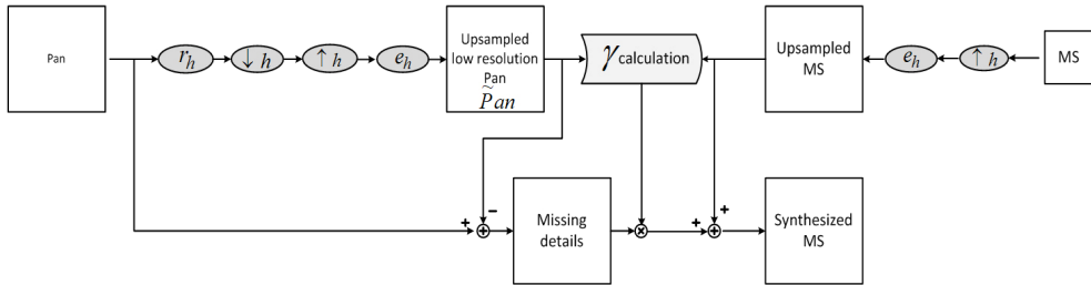
Fig. 5. Blockdiagram of GLP-SDM method
