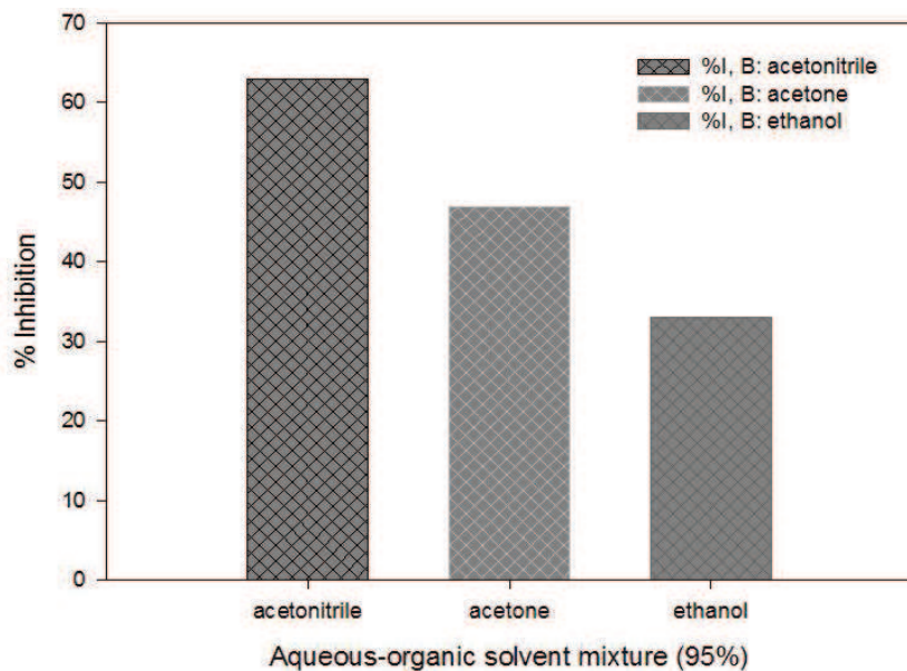
Fig. 2. Results obtained for the inhibition of AChE enzyme activity in the Au/MBT/PANI/AChE/PVAc biosensor after 20 minutes of incubation in 3 different 95% water-organic solvent mixtures. The maximum ATCh substrate concentration was 2.0 mM during the biosensor evaluation.
