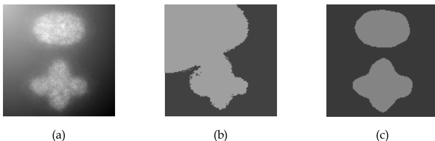
Fig. 12. Segmentation results on the first synthetic image. (a) The synthetic image generated by MOSE. (b) Segmentation by FCM. (c) Segmentation by 2DFCM.
