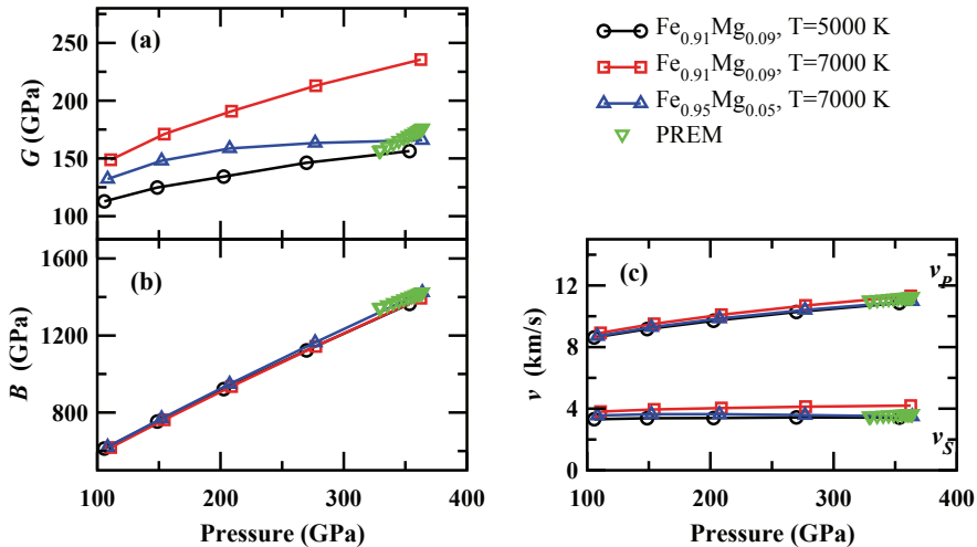
Fig. 11. Shear and bulk moduli, and sound velocities of bcc Fe-Mg alloys. Calculated shear moduli (a), bulk moduli (b) and sound velocities ( v_S shear wave and v_P compressional wave velocities, panel (c)) are displayed for \text{Fe}_{0.91}\text{Mg}_{0.09} at temperatures of T=5000 K (circles) and T=7000 K (squares), and for \text{Fe}_{0.95}\text{Mg}_{0.05} at T=7000 K (triangles). Seismic data as given in the PREM model (Dziewonski & Anderson, 1981) are shown for comparison (inverted triangles).
