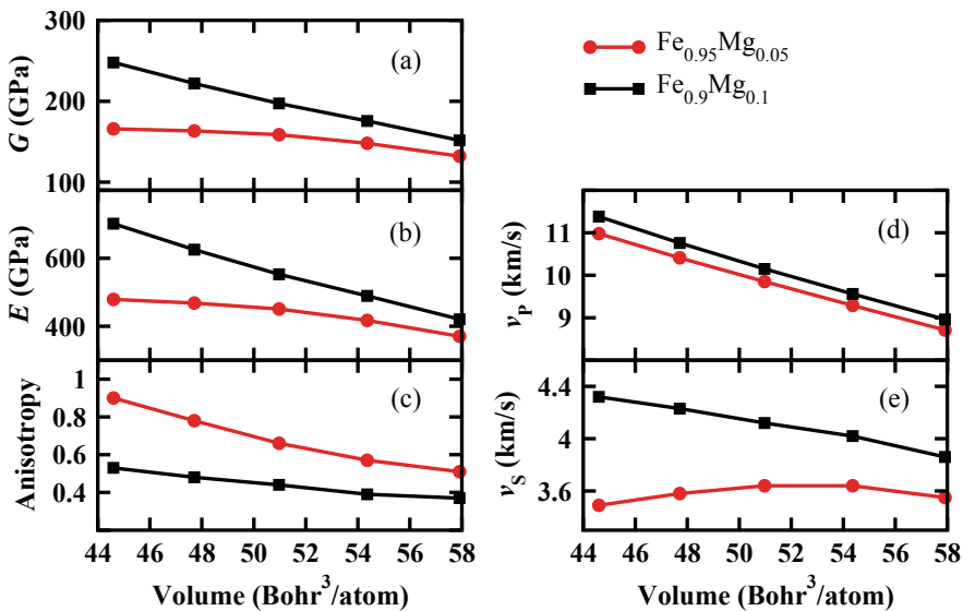
Fig. 10. Shear ( G ) and Young moduli ( E ), polycrystalline anisotropy, and longitudinal ( v_P ) and transversal ( v_S ) sound velocities of bcc \text{Fe}_{0.95}\text{Mg}_{0.05} (red circles) and \text{Fe}_{0.9}\text{Mg}_{0.1} alloys (black squares) at different V volumes, at T=7000 \text{ K} temperature.
