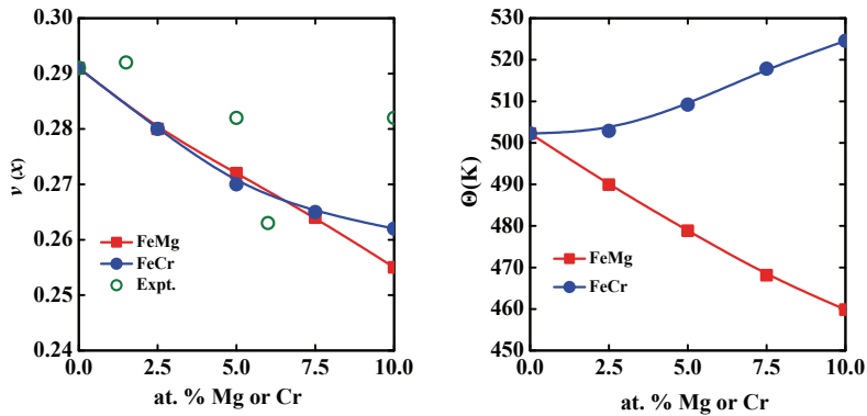
Fig. 4. Theoretical (EMTO) Poisson's ratio (left panel) and Debye temperature (right panel) of ferromagnetic bcc \text{Fe}_{1-x}\text{Mg}_x ( 0 \leq x \leq 0.1 ) random alloys as a function of Mg concentration. For comparison, theoretical and experimental (Speich et al., 1972) Poisson's ratio and Debye temperature for Fe-Cr are also shown.
