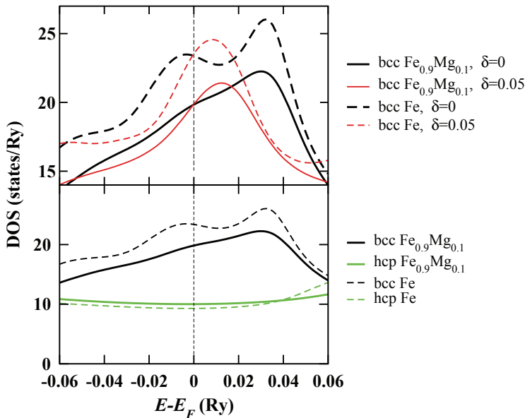
Fig. 9. Electronic density of states of Fe at T=0 K for an energy window corresponding to \sim 5000 - 8000 K. Lower panel: density of states of Fe and \text{Fe}_{0.9}\text{Mg}_{0.1} in the bcc and hcp phases, respectively. Upper panel: density of states for non-distorted bcc Fe and \text{Fe}_{0.9}\text{Mg}_{0.1} ( \delta=0 ) and for distorted bcc Fe and \text{Fe}_{0.9}\text{Mg}_{0.1} ( \delta=0.05 ). Similar orthorhombic distortions have been used to compute the tetragonal cubic shear modulus C' . Vertical dashed lines denote the Fermi level.
