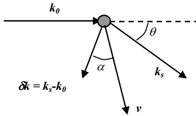
Fig. 7. Principles of LDF. The particle has a velocity v . Vectors k_0 and k_s denote the incoming and scattered light wave vectors, and \delta k is the difference vector.
