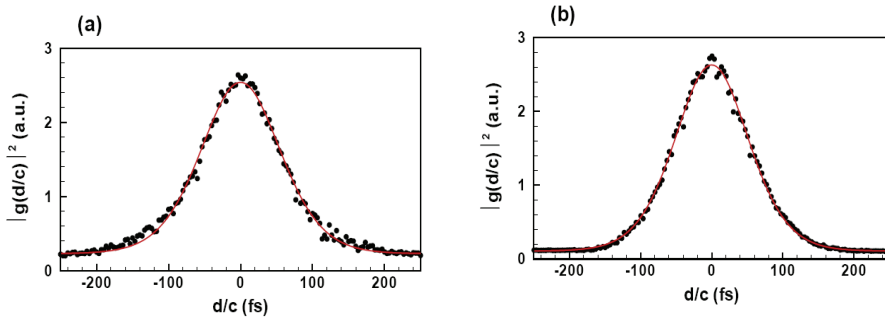
Fig. 7. Measured square of the scaled autocorrelation function (circles) and fitted curve for a hyperbolic-secant temporal pulse-shape (line) versus time delay d/c. (a) larger magnification (see Fig. 5 (a)) and (b) smaller magnification (see Fig. 5(b)).
