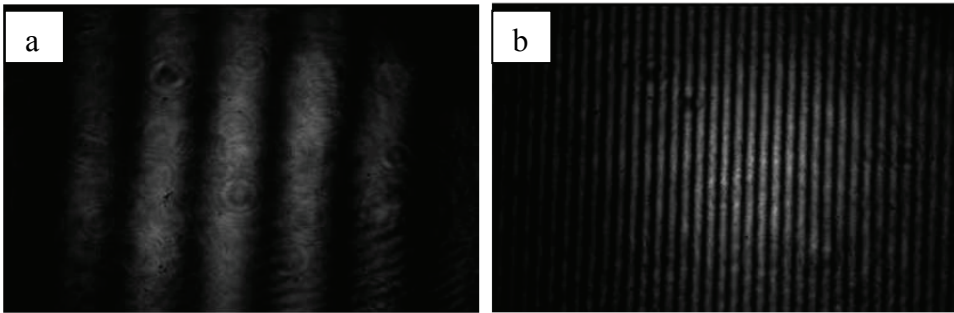
Fig. 5. Images of interference patters. The camera lens magnification used is \times 6 larger for (a) the image on the left than (b) for the image on the right. The distance perpendicular to the fringes amounts to 0.6 mm and 3.6 mm, respectively.
