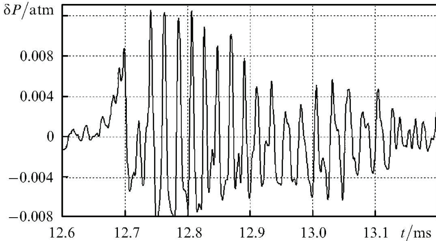
Fig. 6. Pressure pulsations \delta P in the OPD produced by pulse trains with \phi = 1.1 \text{ kHz} , f = 50 \text{ kHz} , W = 720 \text{ W} , N = 15 , V = 300 \text{ m s}^{-1} , D_r = 1.5 \text{ cm} , H = 5 \text{ cm} , D_j = 4 \text{ mm} , and F = 4.5 \text{ g} .
