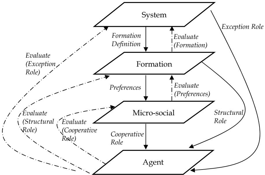
Fig. 2. The 4-layers MRCC Model.
