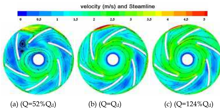
Fig. 11. Steady flow calculation results of relative velocity and streamlines in impeller at t=0 (a) At small flow rate case (b) At design flow rate case (c) At large flow rate case
