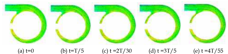
Fig. 5. The absolute velocity and streamlines in volute at design flow rate condition ( Q=Q_d )
