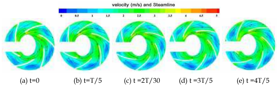
Fig. 4. Relative velocity and streamlines in impeller at design flow rate condition ( Q=Q_d )
