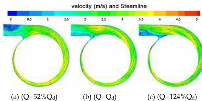
Fig. 13. Steady flow calculation results of absolute velocity and streamlines in volute at t=0 (a) At small flow rate case (b) At design flow rate case (c) At large flow rate case
