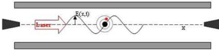
Fig. 1. (Color online) A sketch of a two-level ion trapped in one-dimensional electromagnetic trap (Only the vibrational motion along the x -direction is considered) and driven by a classical laser field propagating along the x direction.
