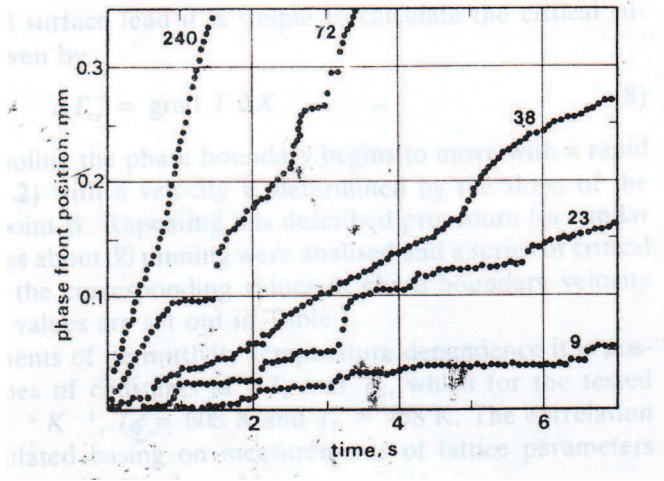
Fig. 2. The position of phase boundary as a function of time for \text{NaNbO}_3 single crystal for the various values of average velocity v_a (the values in \mu\text{ m/s} given against the curves). (Dec & Yurkevich, 1990).
