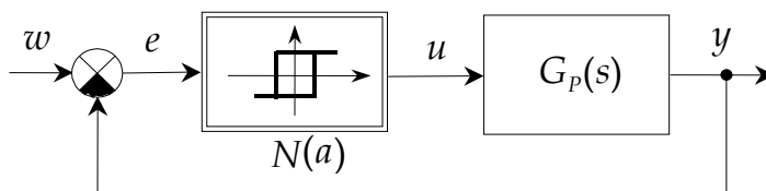
Fig. 1. Closed-loop system with two-position relay
