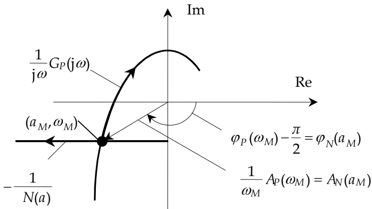
Fig. 6. Geometric interpretation of relay method with integrator
