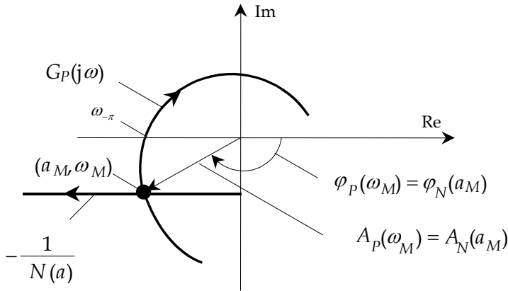
Fig. 3. Geometric interpretation of relay method without integrator
