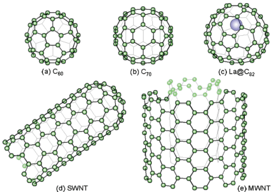
Fig. 2. Carbon nano-materials
