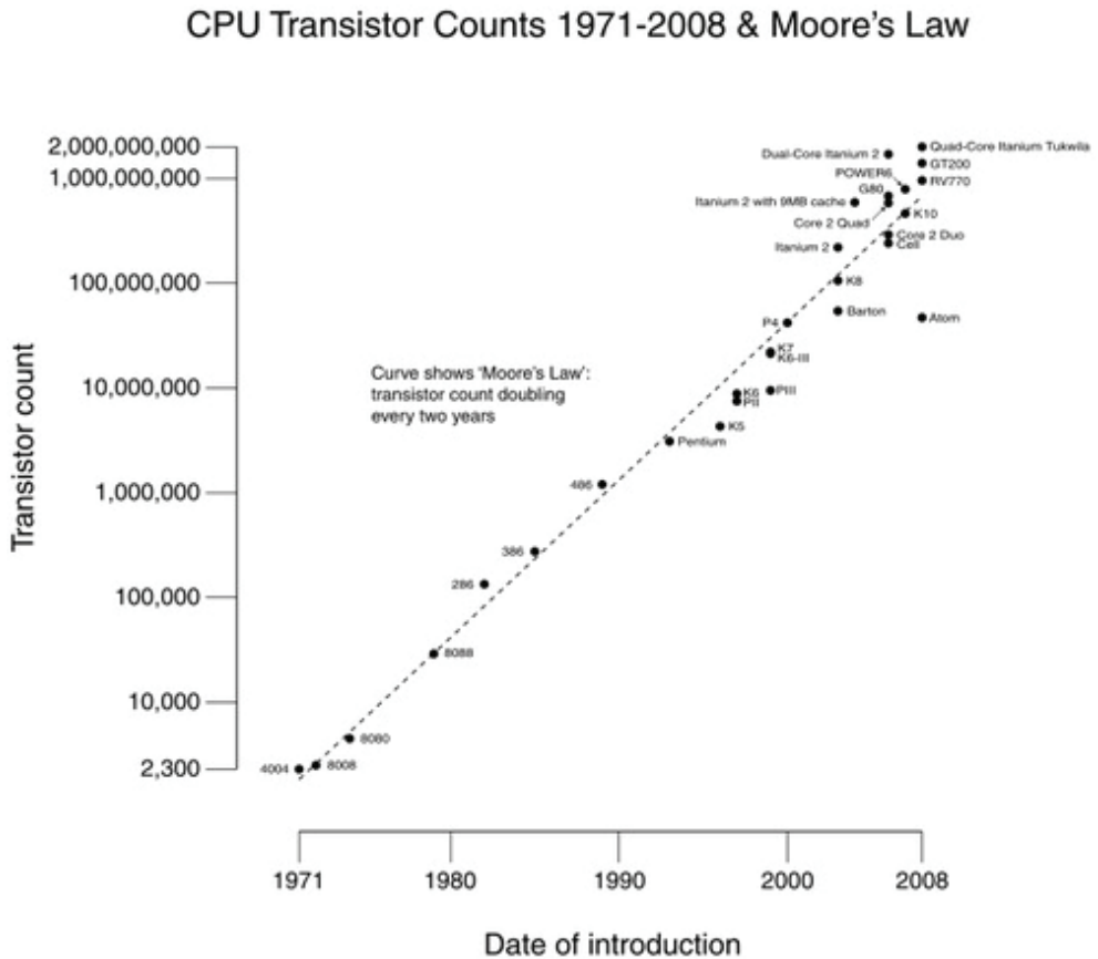
Fig. 1. Moore's law from Intel's history (Intel HP)
