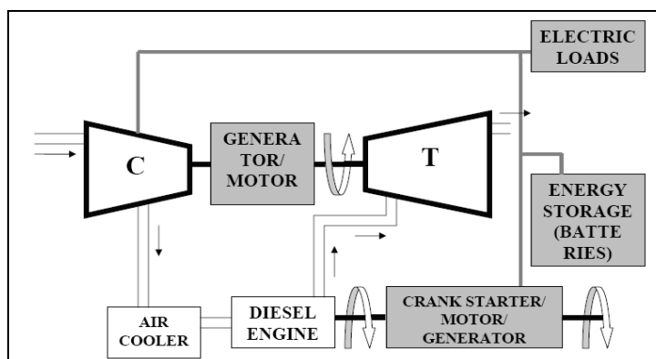
Fig. 7. Schematic view of Electrical Turbocompounding.
