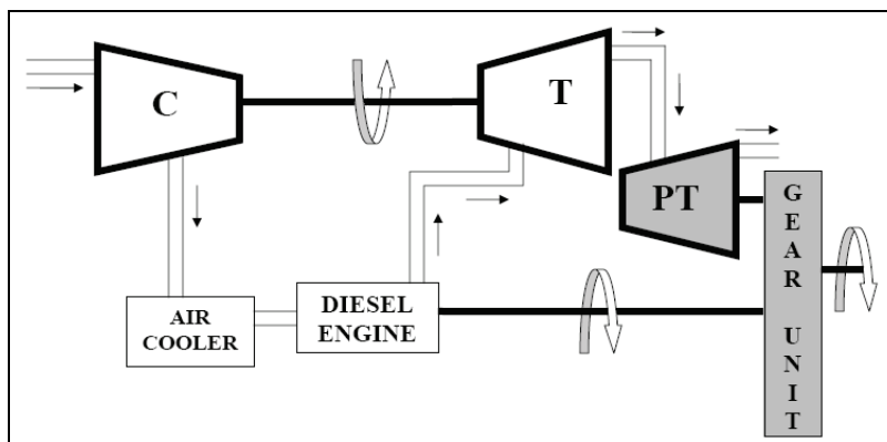
Fig. 1. Schematic view of Mechanical Turbocharging.
