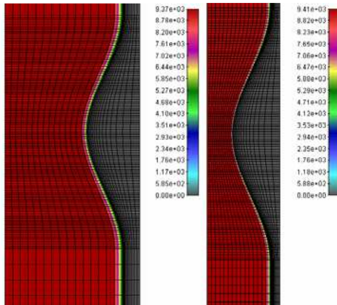
Fig. 4. a) Pressure distribution for an initial mild stenosis 30% constriction by area b) Pressure distribution at the end of stenosis process after 10^7 sec[units Pa]
