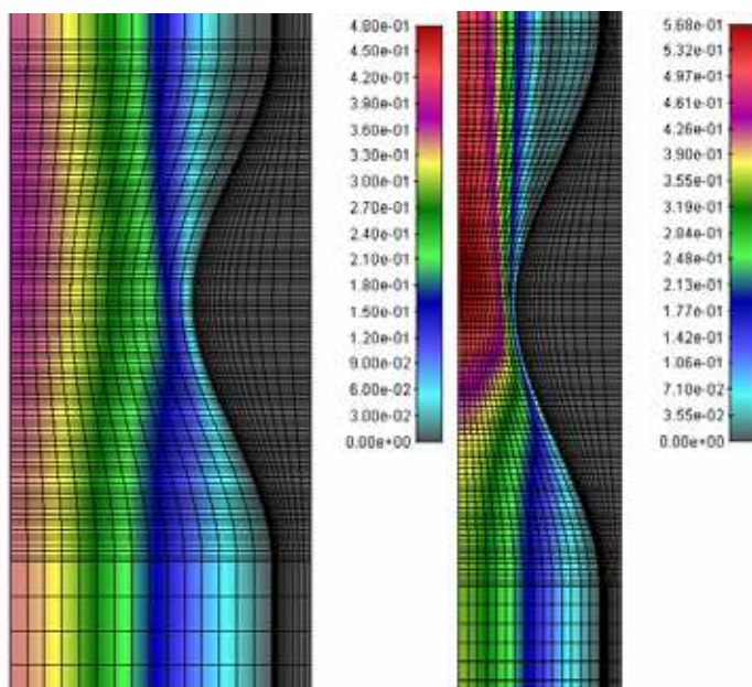
Fig. 3. a) Velocity distribution for an initial mild stenosis 30% constriction by area b) Velocity distribution at the end of stenosis process after 10^7 sec [units m/s]
