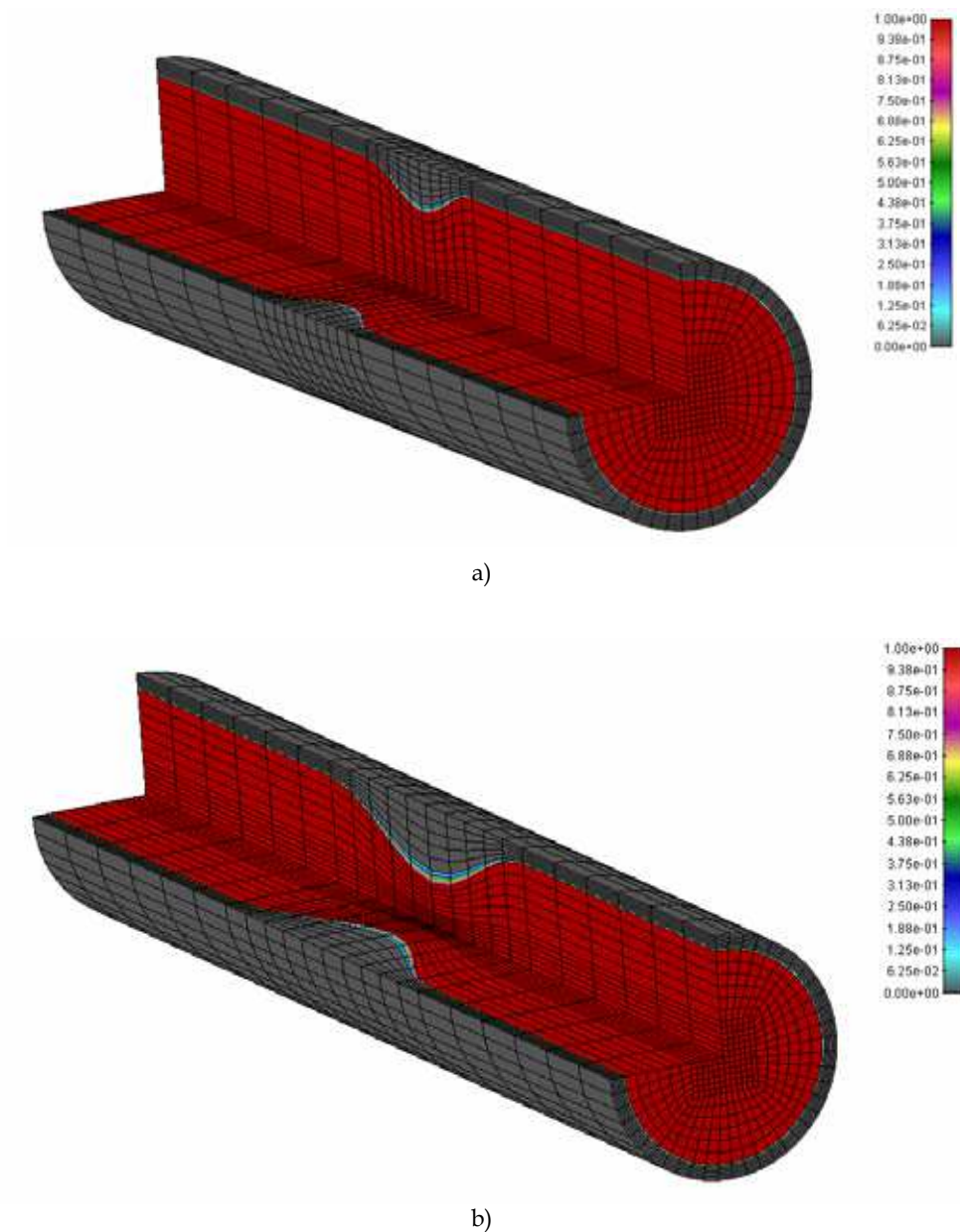
Fig. 14. a) Lumen LDL distribution for an initial mild stenosis 30% constriction by area b) Lumen LDL distribution at the end of stenosis process after 10^7 sec [units mg/mL]
