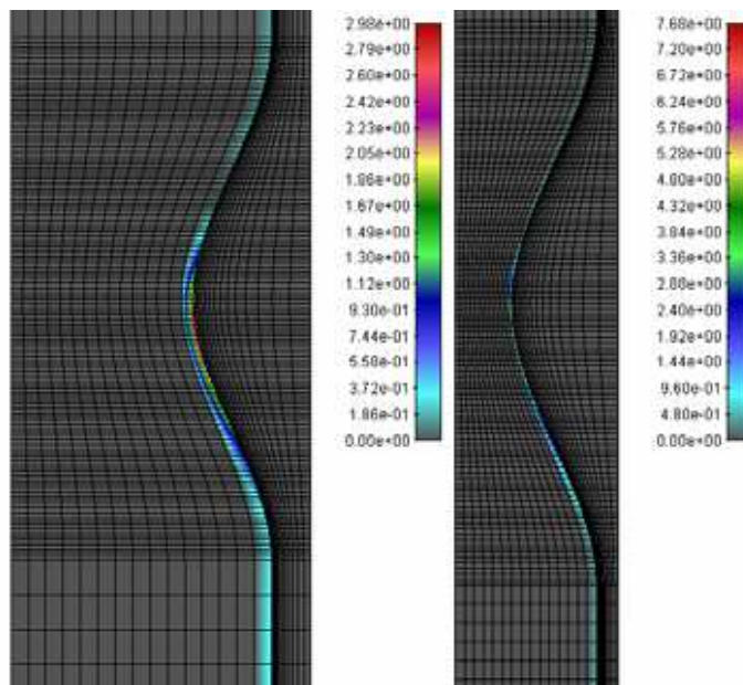
Fig. 5. a) Shear stress distribution for an initial mild stenosis 30% constriction by area b) Shear stress distribution at the end of stenosis process after 10^7 sec[unitsdyn/cm 2 ]
