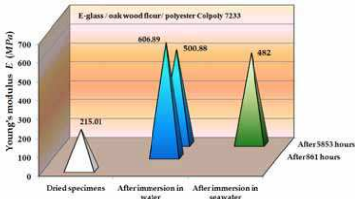
Fig. 30. The effects of water /seawater absorption on Young's modulus E in case of E-glass EWR145 / oak wood flour / polyester Copoly 7233
