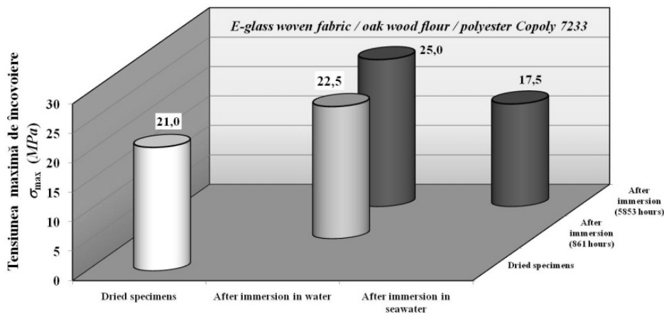
Fig. 31. The effects of water /seawater absorption on on the maximum flexural stress \sigma_{max} in case of E-glass EWR145 / oak wood flour / polyester Copoly 7233
