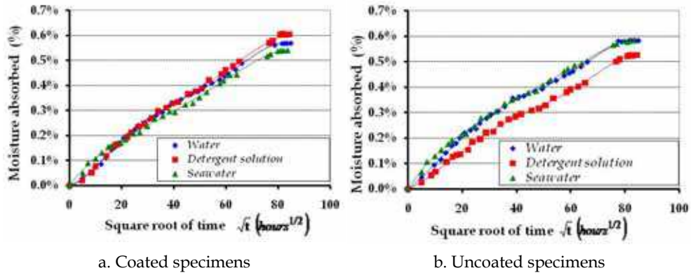
Fig. 6. Absorption data in case of E-glass / Heliopol 8431 ATX composite material
