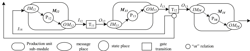
Fig. 8. A conflict model in T_{12}
