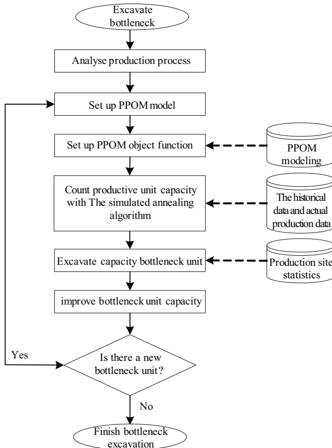
Fig. 2. Bottleneck detecting process based on PPOM
