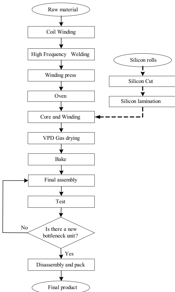
Fig. 6. Power Transformer production process of M company
