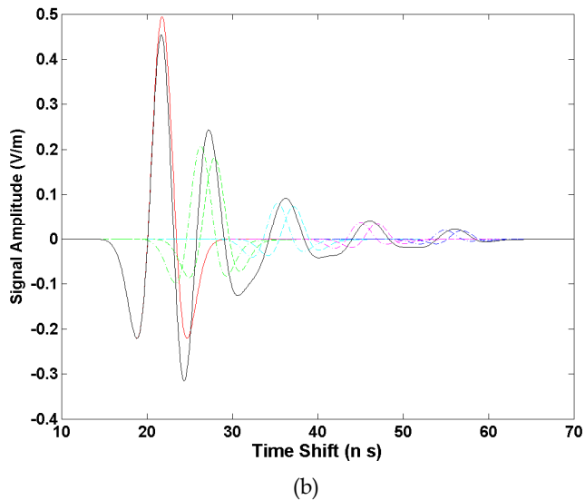
Fig. 5. Waveforms of direct field, reflected fields and their summations at receiver. (a) horizontal polarization; (b) vertical polarization.
