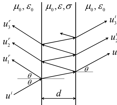
Fig. 7. Pulse is impinging on lossy dielectric slab.
