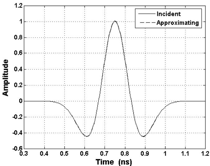
Fig. 1. Incident pulse and approximating pulse with 40 exponentials.
