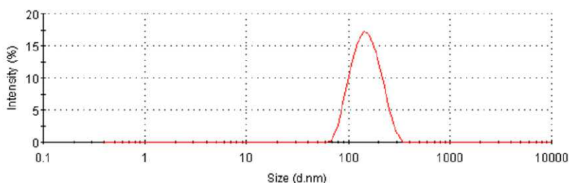
Fig. 5. Size distributions of (a) DiO and (b) perylene nanocrystals dispersed in water. The peak sizes of the DiO particles were 22 nm (intensity: 58%) and 146 nm (intensity: 42%); the peak size of the perylene particles was 155 nm (intensity: 100%; i.e., monodispersity).
