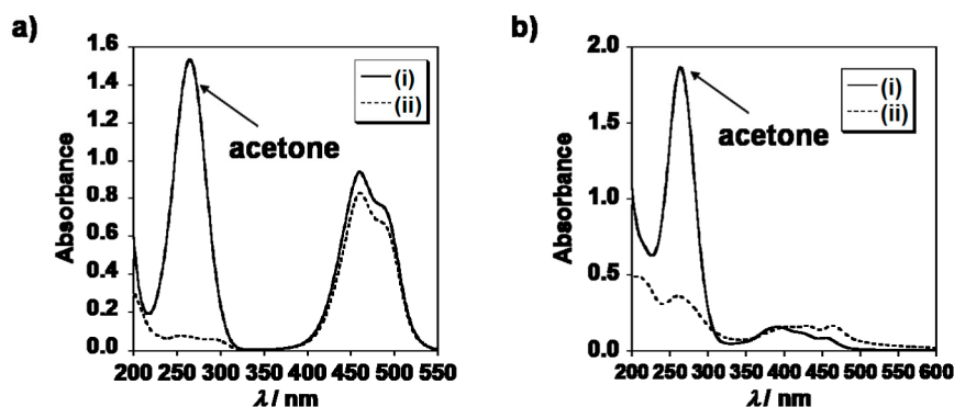
Fig. 4. Absorption spectra of water dispersions of (a) DiO nanocrystals and (b) perylene nanocrystals. (i) before and (ii) after dialysis. The disappearances of the absorbance of acetone (at \lambda_{\max} = 265 nm) were confirmed.
