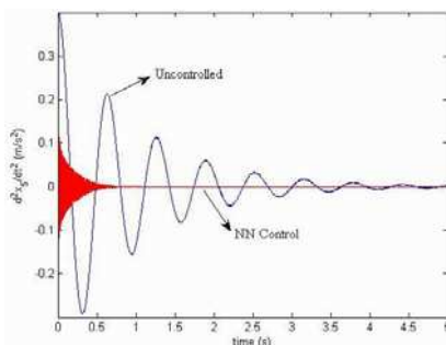
Fig. 10. Time responses of passenger seat vertical acceleration.
