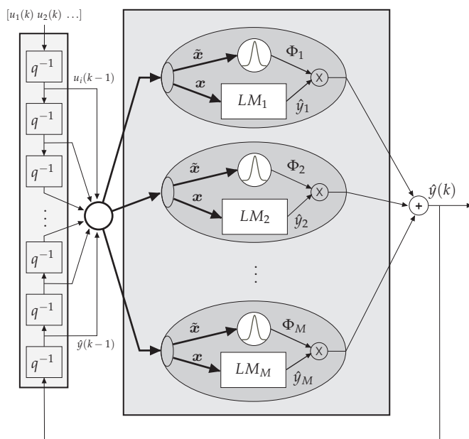
Fig. 2. Architecture of a dynamic local model network
