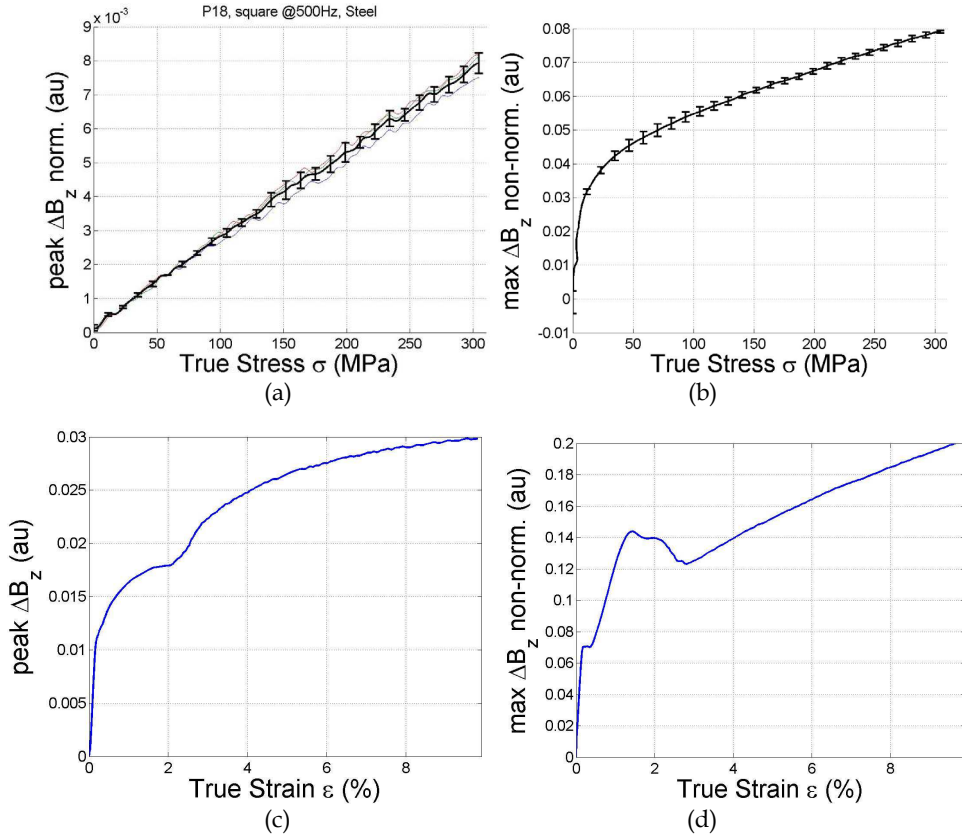
Fig. 4. Results of PEC measurements on steel under elastic and plastic deformation; a) Normalised PEC response peak(\Delta B_z^{NORM}) , under elastic stress; (b) Non-normalised PEC response max(\Delta B_z^{NON-NORM}) under elastic stress, a) Normalised PEC response peak(\Delta B_z^{NORM}) under plastic strain (b) Non-normalised PEC response max(\Delta B_z^{NON-NORM}) under plastic strain
