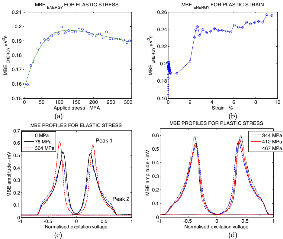
Fig. 5. Results of MBE measurements on steel under elastic and plastic deformation; a) MBE_{ENERGY} for elastic stress, b) MBE_{ENERGY} for plastic strain, c) MBE profiles for elastic stress, d) MBE profiles for plastic stress
