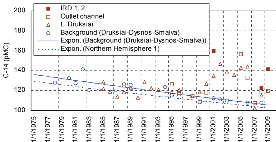
Fig. 6. The 14 C specific activity of DIC in water bodies related to INPP at short distance from INPP for the period 1975–2009, compared with 14 C activity in air of Northern Hemisphere according to Hua & Barbetti (2004) and with local background 14 C level
