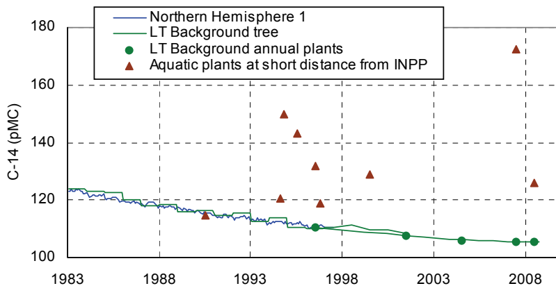
Fig. 7. The 14 C specific activity of aquatic plants at short distance from INPP, compared with 14 C activity in air of Northern Hemisphere according to Hua & Barbetti (2004) and with local background 14 C level
