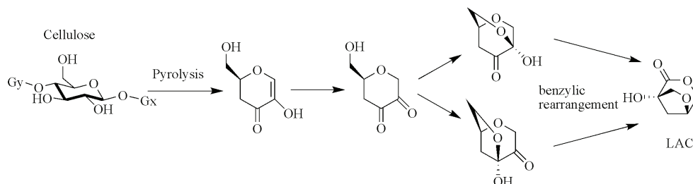
Fig. 6. The pyrolytic pathways for the formation of LAC from pyrolysis of cellulose (Torri et al., 2009b). As been indicated above, the utilization of solid catalysts will provide a convenient way for the catalyst recycles. Further studies have also been conducted by them to use the LAC as a possible building block in the synthesis of fine chemicals.
