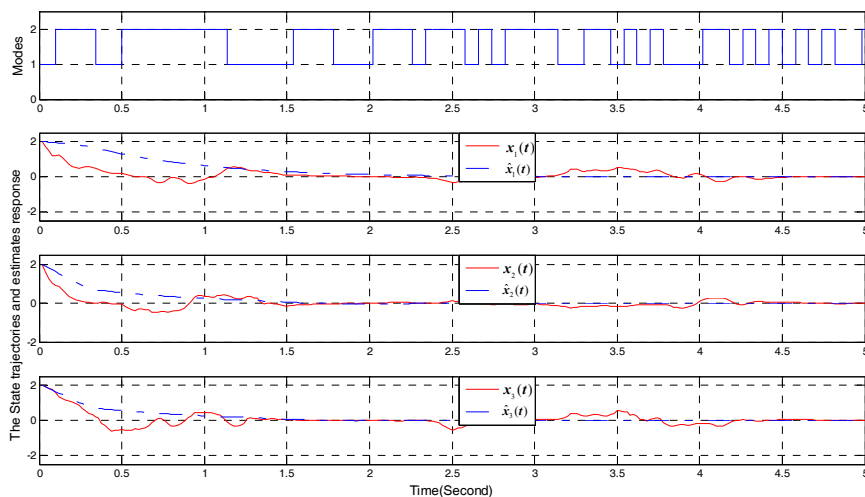
Fig. 3. The state trajectories and estimates response
