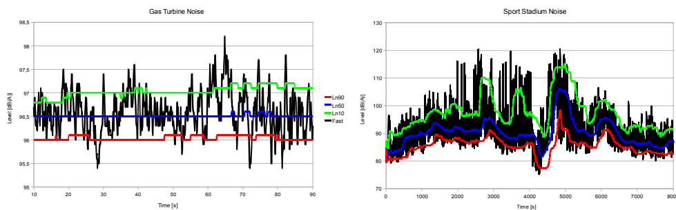
Fig. 7 and 8. Time evolution of percentile Ln levels from a running gas turbine, and time evolution of percentile Ln levels from noise in a sports arena
