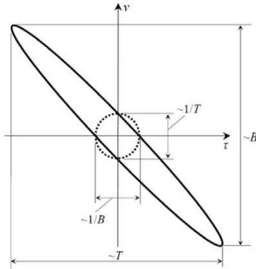
Fig. 2-2. Comparison of contours of ambiguity functions for LFM signal (solid line ellipse) and biphase-coded signal (dotted line circle) having the same pulse duration and bandwidth
