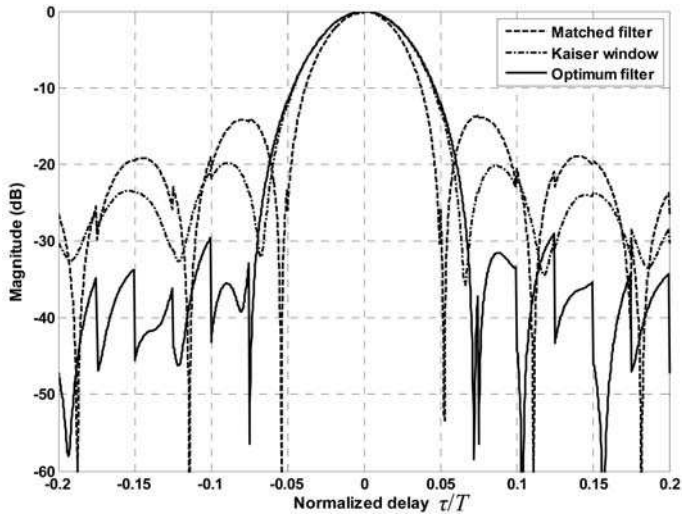
Fig. 2-6. Zero-Doppler cuts of digital cross-ambiguity functions for the optimum filter ( M=N=40 , m=g=2 , v_{max}/B = 0.1 ) and Kaiser window and zero-Doppler cut of digital ambiguity function for the matched filter
