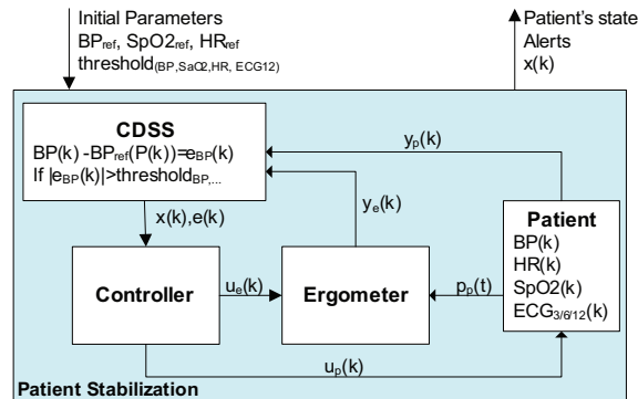
Fig. 6. Control loop for patient stabilization
