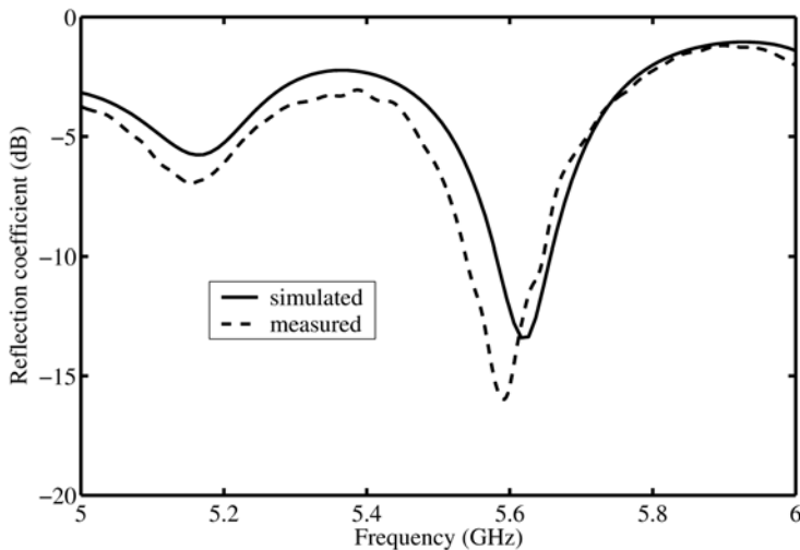
Fig. 17. Simulated and measured reflection coefficient vs. frequency.
