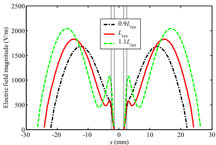
Fig. 2. Magnitude of electric field of isolated slots with half-lengths in vicinity of second-resonance half-length L_{res} . L_{res} = 21.75 mm, W = 1 mm, l_s = 19.4 mm = 0.48 \lambda_{CPW} , h = 1.575 mm, \epsilon_r = 2.33 , w = 3 mm, s = 1 mm. Vertical lines correspond to position of CPW.
