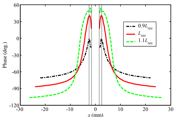
Fig. 3. Phase of electric field of isolated slots with half-lengths in vicinity of second-resonance half-length L_{res} . L_{res} = 21.75 mm, W = 1 mm, l_s = 19.4 mm = 0.48 \lambda_{CPW} , h = 1.575 mm, \epsilon_r = 2.33 , w = 3 mm, s = 1 mm. Vertical lines correspond to position of CPW.
