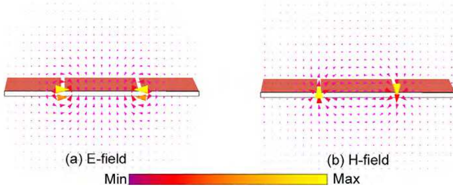
Fig. 6. The transverse electric- (a) and magnetic- (b) field in CPW.
