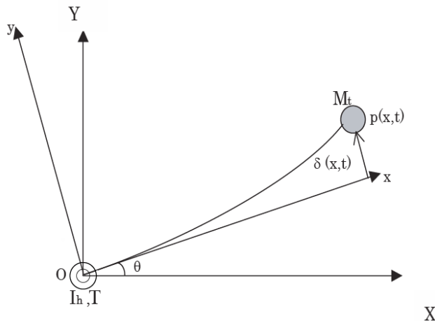
Fig. 1. Flexible arm system.
